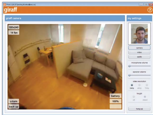
Figure 3. Software version 2.0 of the Pilot interface.
