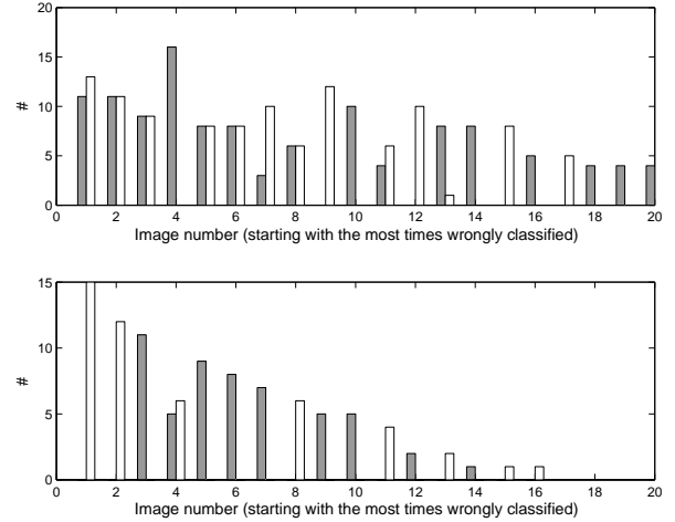
Fig. 4. Distribution of the 20 most frequently wrongly classified images from AdaBoost (gray) and BOC (white), using image size 120 (upper) and 240 (lower).
