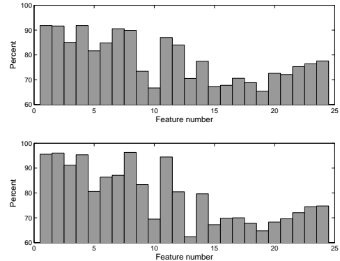
Fig. 3. Histogram of classification rate of individual features in Test 2 as an average of 100 runs with T = 1 , image size 120 (upper) and 240 (lower).
