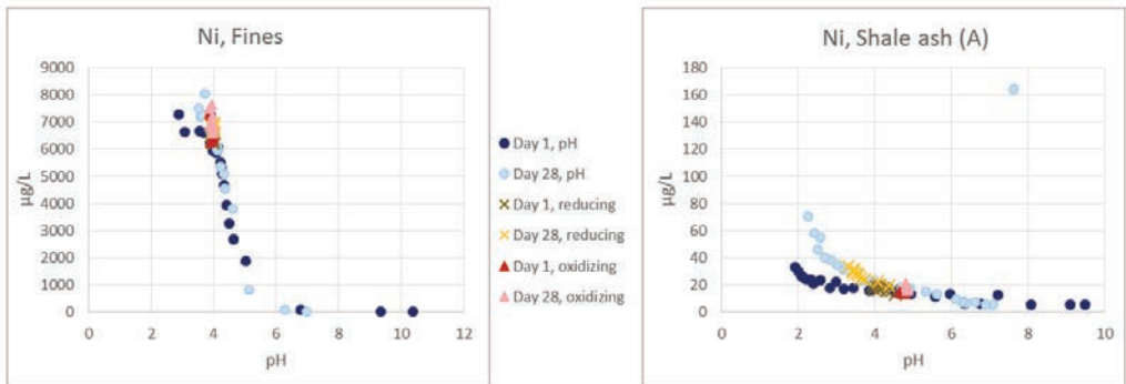
Figure 4 Leaching of nickel was favoured by low pH and showed no impact from manipulation of the redox potential.
